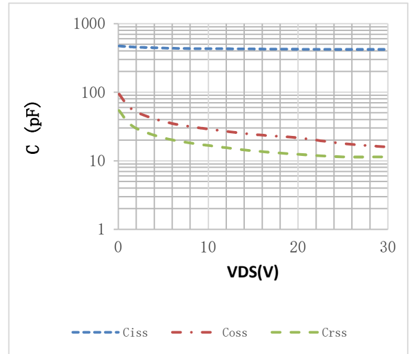
Fig.2 Capacitance Characteristics
